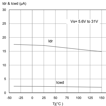
Figure 19. Idr & IcdW vs. Tj
