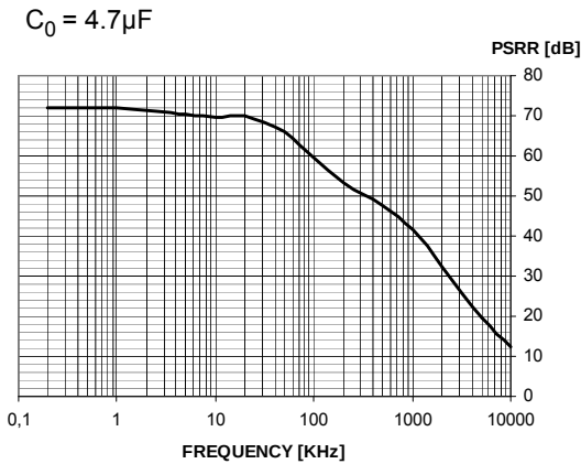
Figure 21. PSRR
