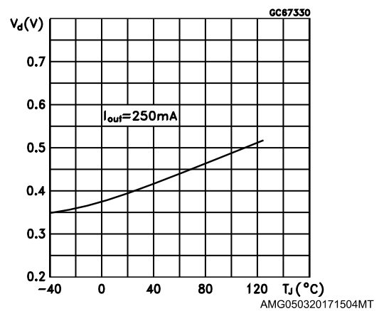
Figure 5: Dropout voltage vs temperature
