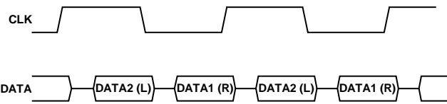
Figure 7. Stereo PDM Format
