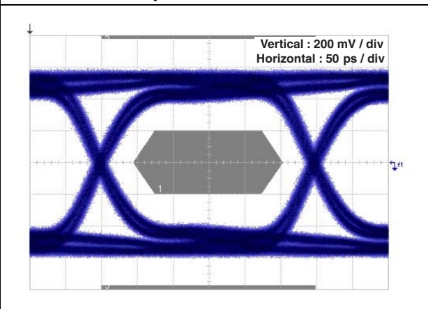
Figure 5. Eye diagram, HDMI mask, at 3.4 Gbps per channel (1)
