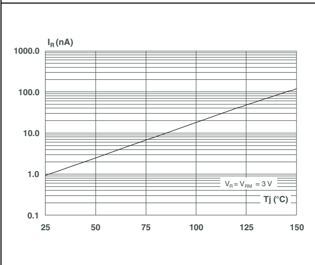
Figure 2. Leakage current versus junction temperature (typical values)
