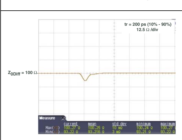
Figure 4. Differential impedance ( Z_{diff} ) (1)
