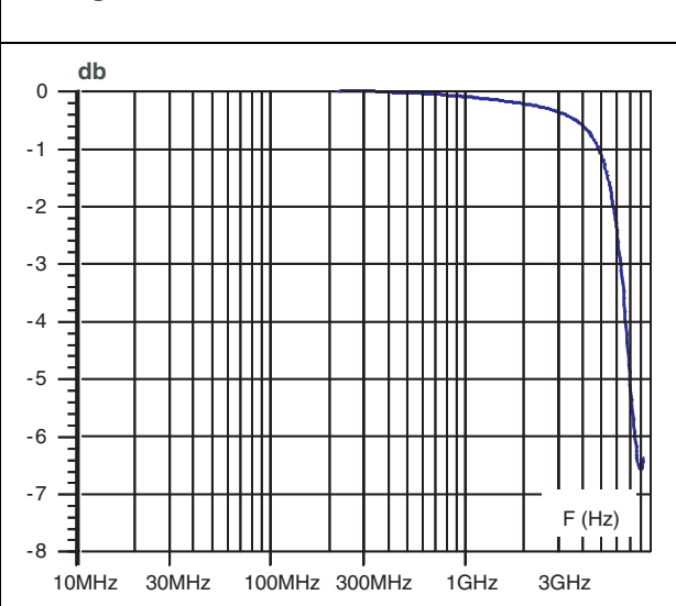
Figure 3. S21 attenuation measurement
