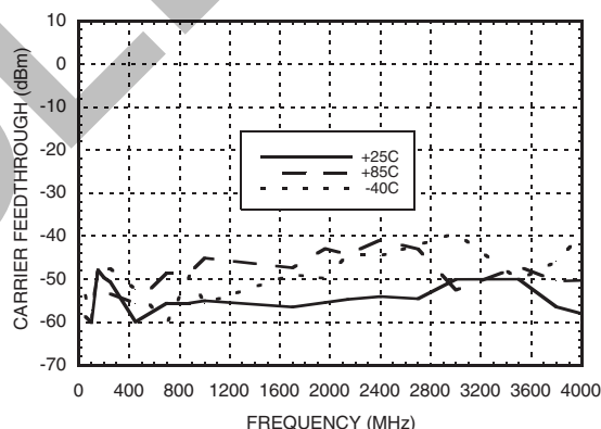
Calibrated Carrier Feedthrough [1] vs. Frequency
