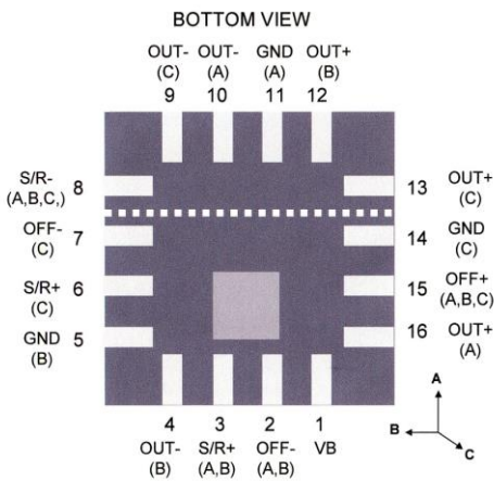
HMC1053 Pinout
