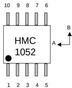
HMC1052 Pinout
