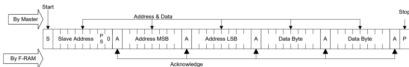
Figure 9. Multi-Byte Write
