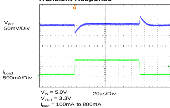
Transient Response
