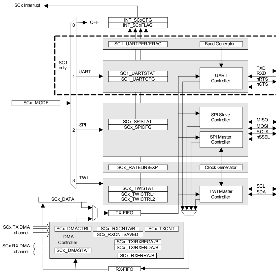
Figure 8.1. Serial Controller Block Diagram
