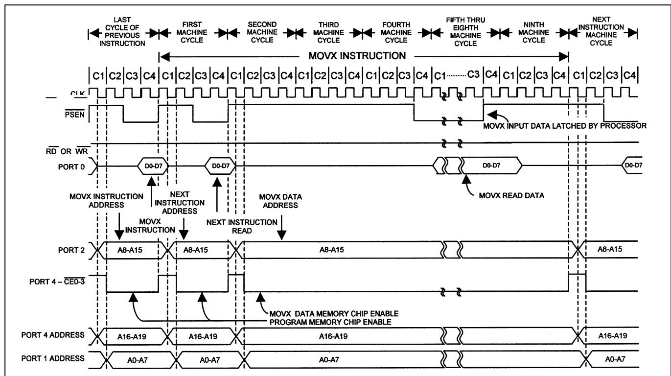
Figure 23. Nonmultiplexed 9-Cycle Data Memory \overline{\text{CE0-3}} Read
