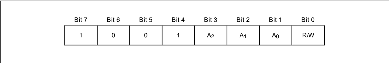
Figure 7. Address Byte
