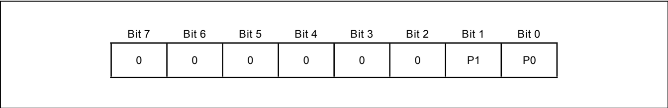
Figure 8. Pointer Byte
