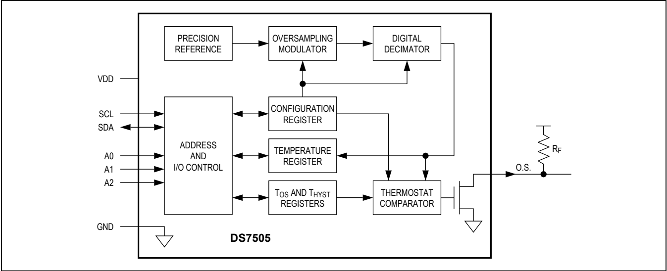
Figure 2. Block Diagram
