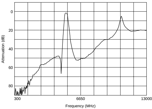
Spurious: DFCB35G25LAHAA
