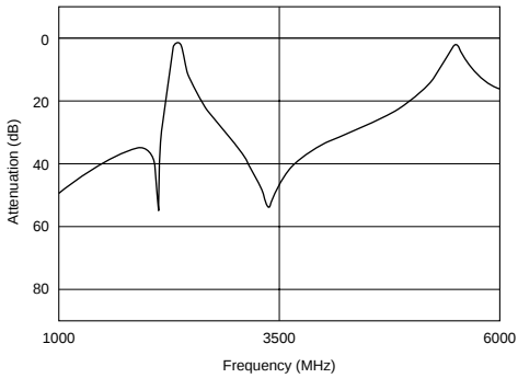
Spurious: DFCB22G33LBJAA
