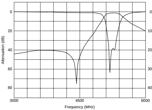
Pass Band: DFCB25G25LAHAA
