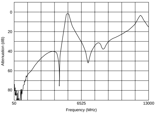
Spurious: DFCB25G25LAHAA
