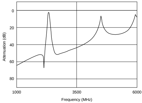
Spurious: DFCB32G33LBJAA
