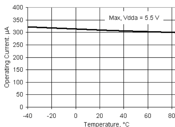
Figure 11-47. VDAC Operating Current vs Temperature, 1 V Mode, High speed mode
