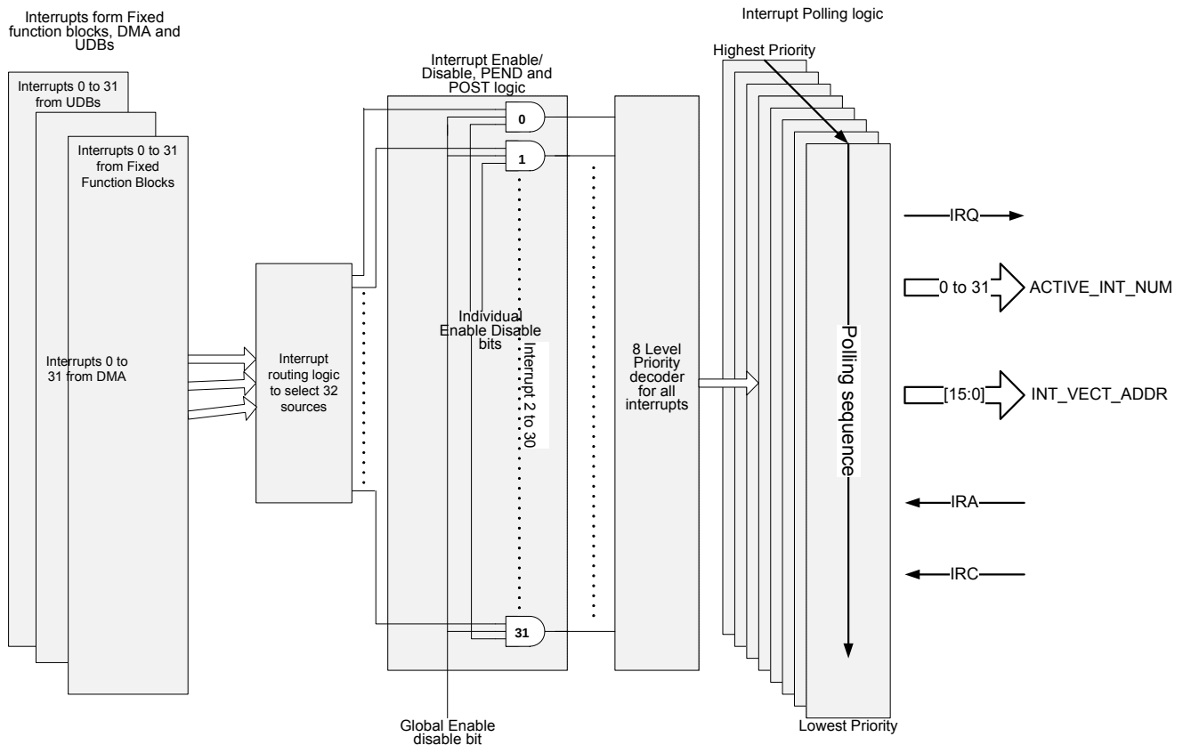
Figure 4-3. Interrupt Structure
