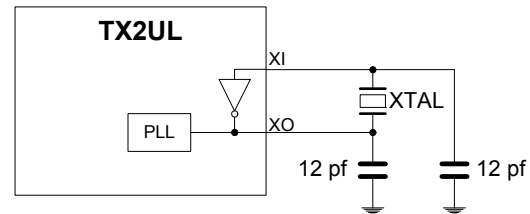
Figure 2. Crystal Configuration
