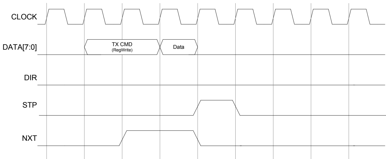
Figure 11. Register Write
