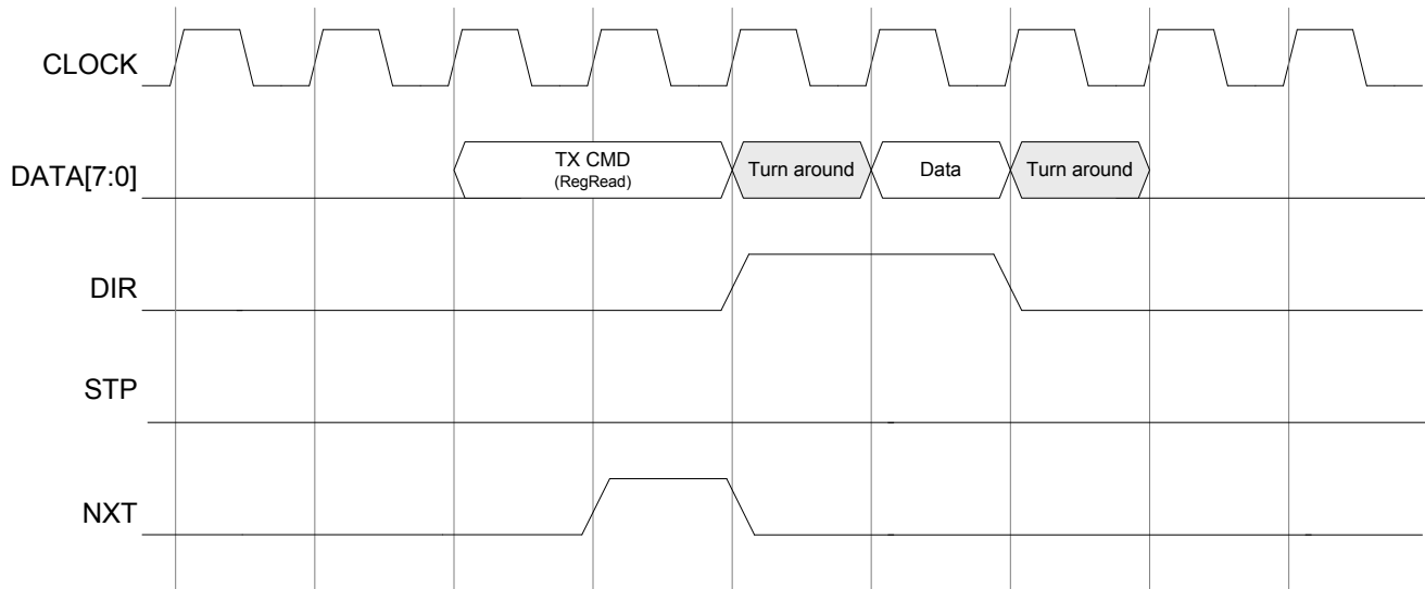
Figure 12. Register Read
