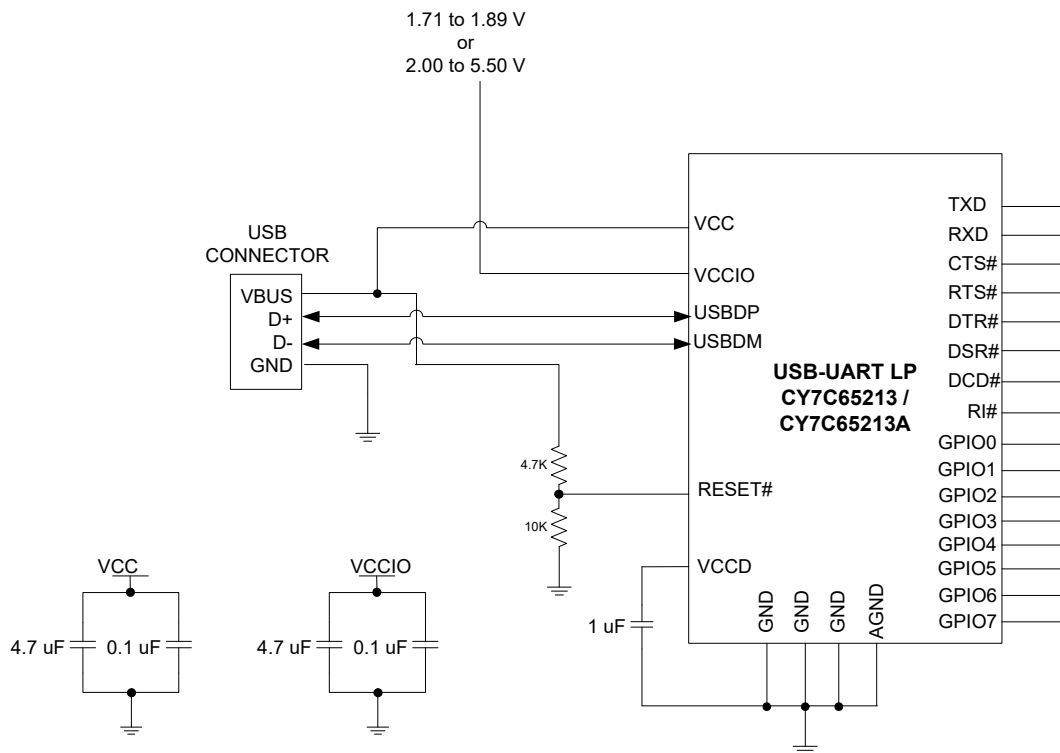
Figure 2. Self-Powered Configuration
