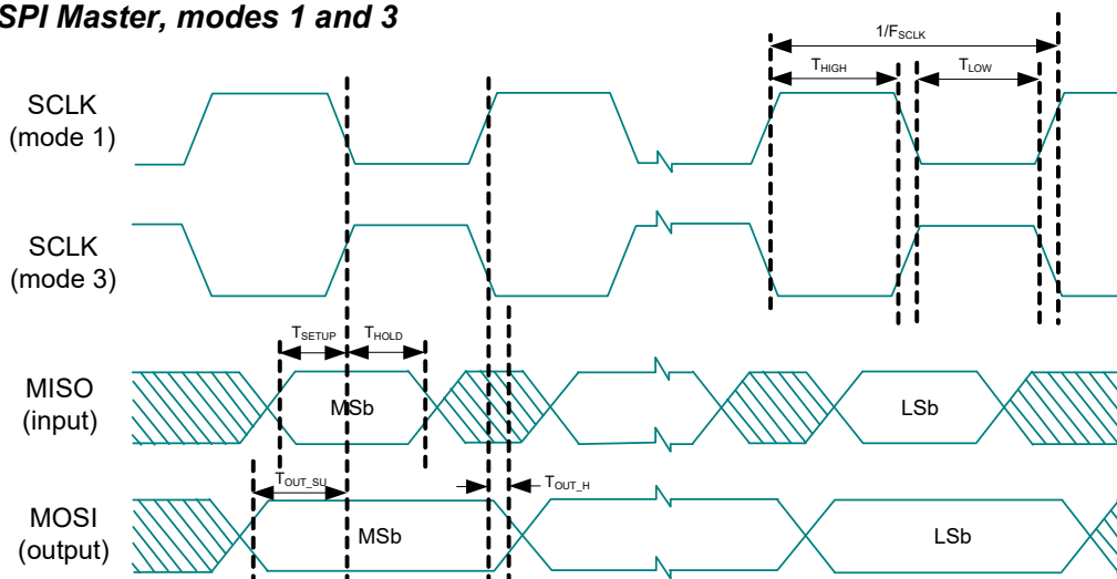
SPI Master, modes 1 and 3
