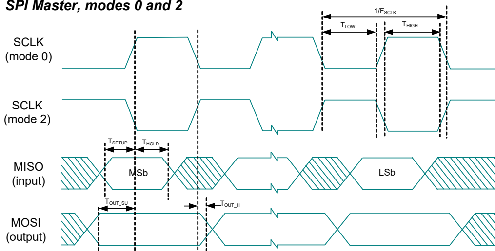
SPI Master, modes 0 and 2
