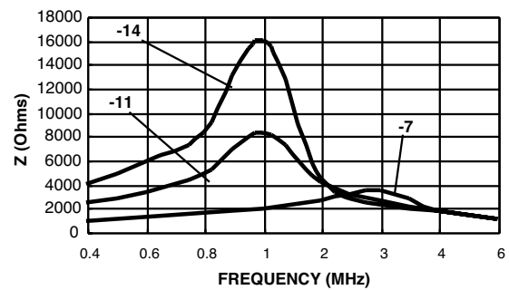
Impedance CMS3 - 7,11, & 14
