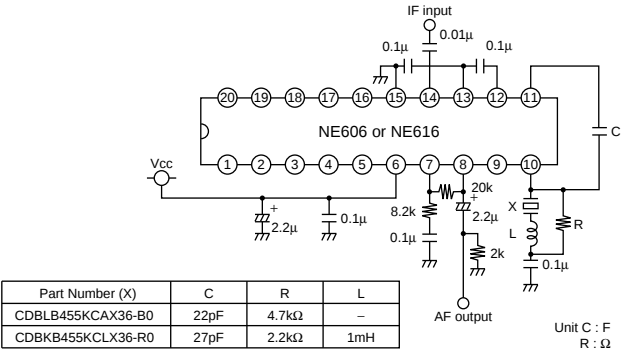
NE(SA)606/616
