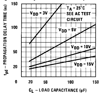
Propagation Delay Time vs. Load Capacitance
