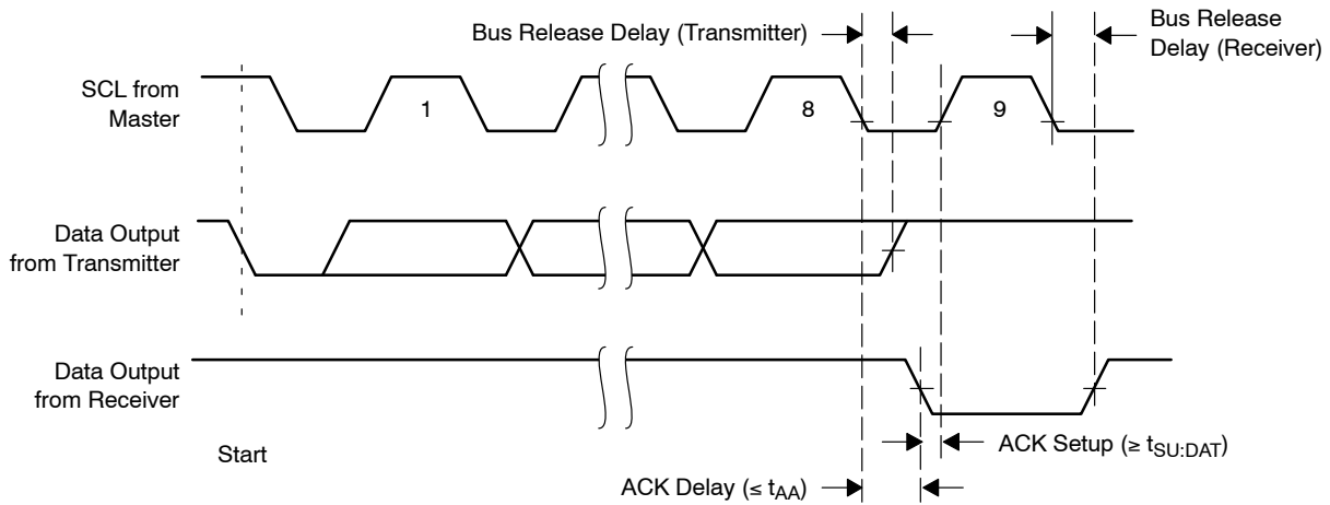
Figure 4. Acknowledge Timing
