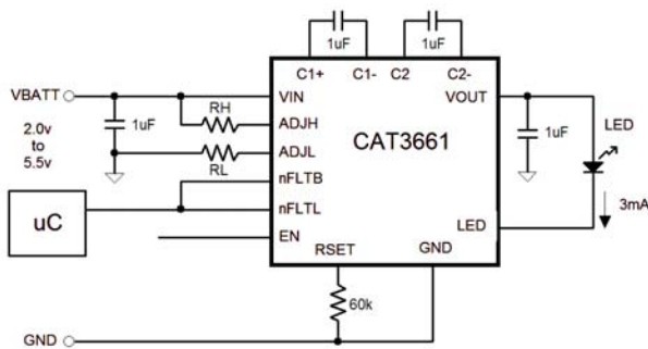
Figure 25. Application Circuit with R H & R L
