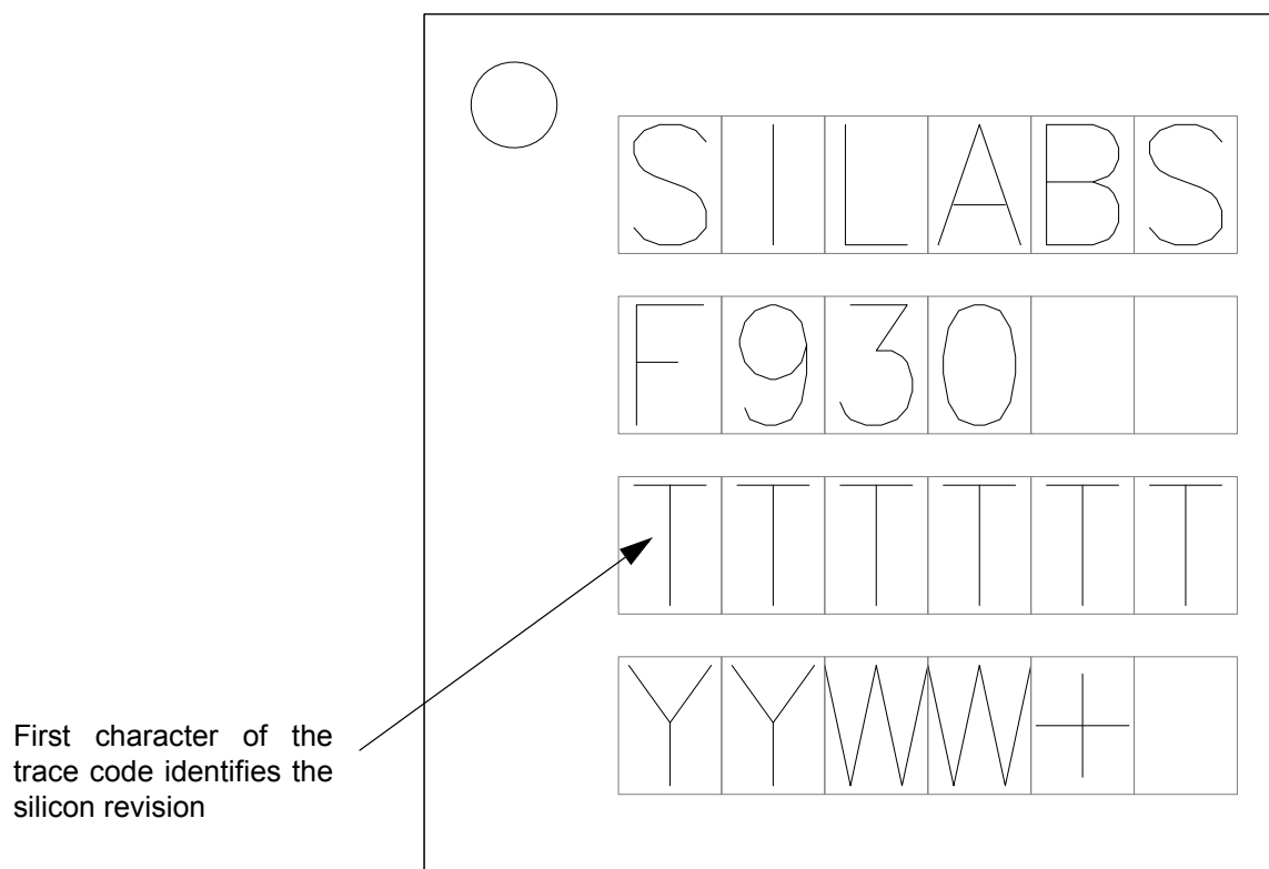
Figure 3.4. QFN-32 Package Marking Diagram
