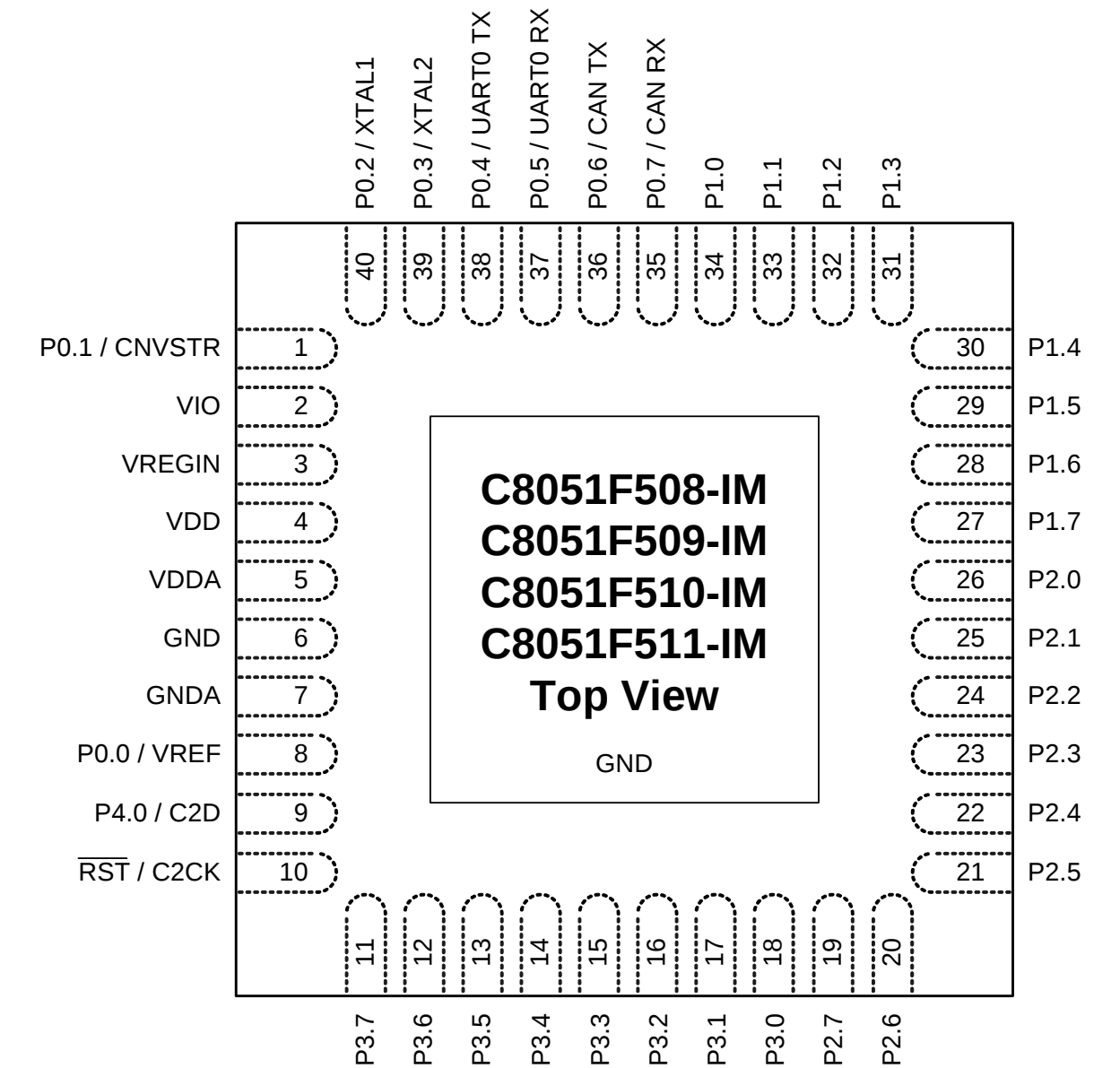
Figure 3.3. QFN-40 Pinout Diagram (Top View)
