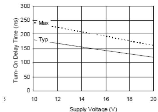
Figure 6B. Turn-On Delay Time vs. Supply Voltage
