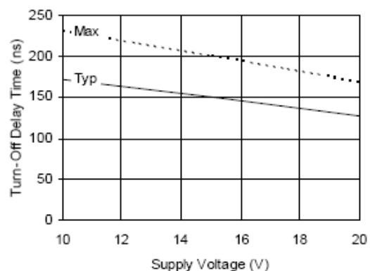
Figure 7B. Turn-Off Delay Time vs. Supply Voltage
