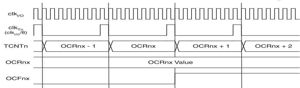
Figure 15-10. Timer/Counter Timing Diagram, Setting of OCF2A, with Prescaler ( f_{clk\_I/O}/8 )
