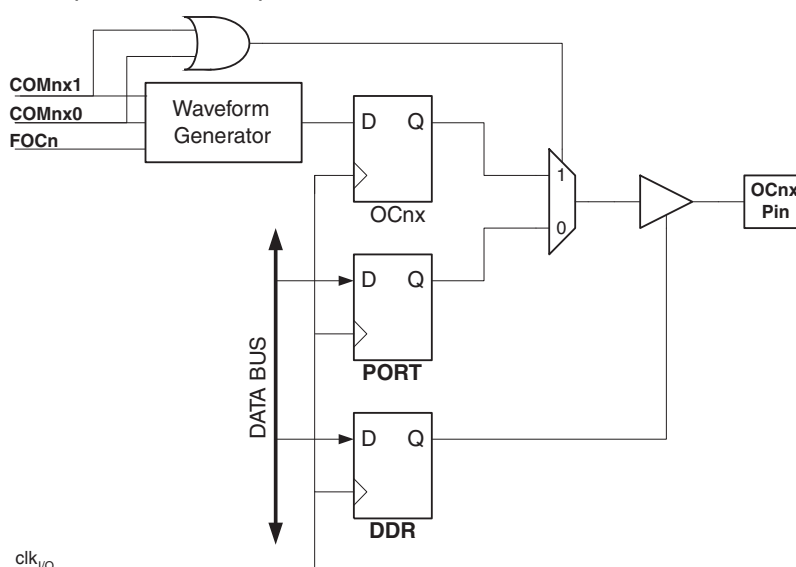
Figure 12-4. Compare Match Output Unit, Schematic
