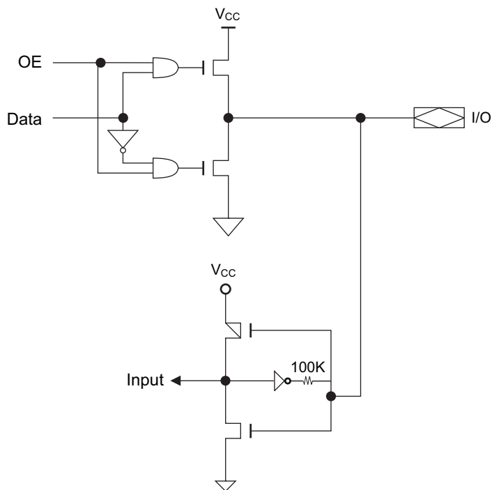
Figure 6-2. I/O Diagram
