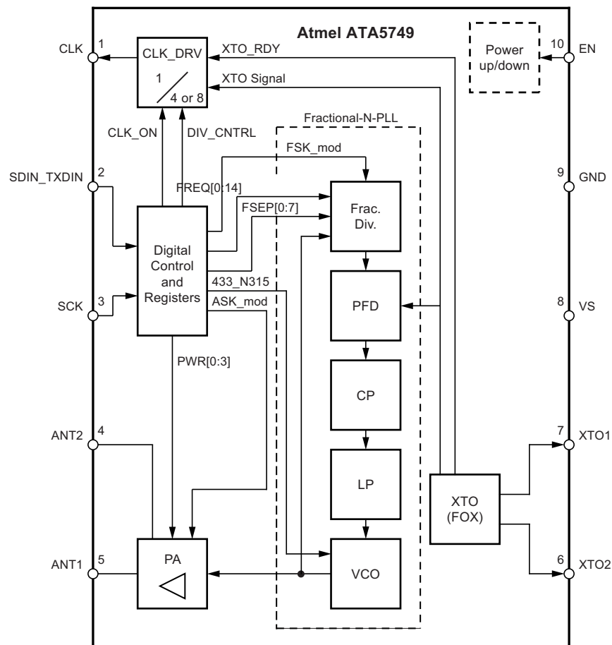
Figure 1-1. Block Diagram
