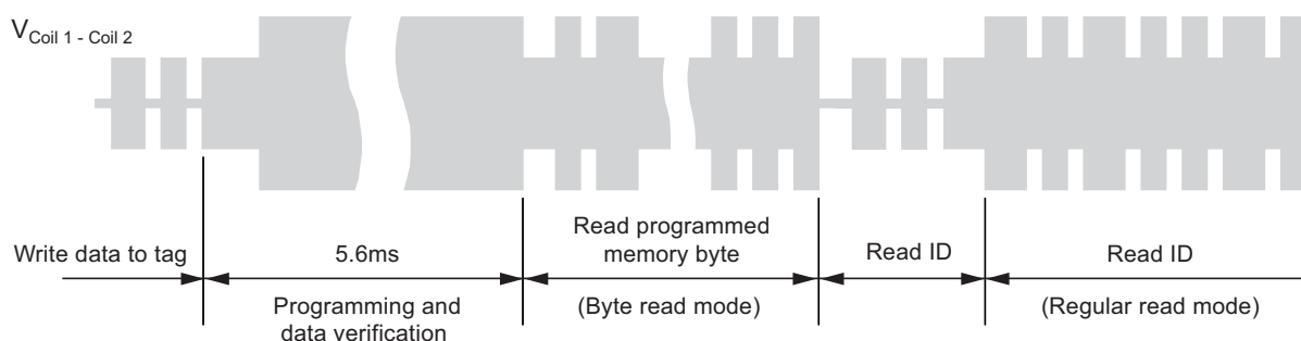
Figure 5-5. Coil Voltage after Programming a Byte
