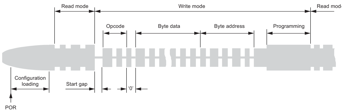
Figure 5-3. Complete Write Sequence
