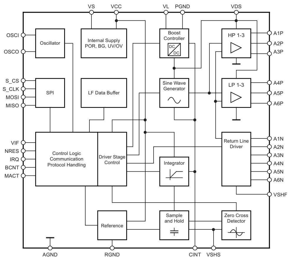
Figure 1-1. Block Diagram
