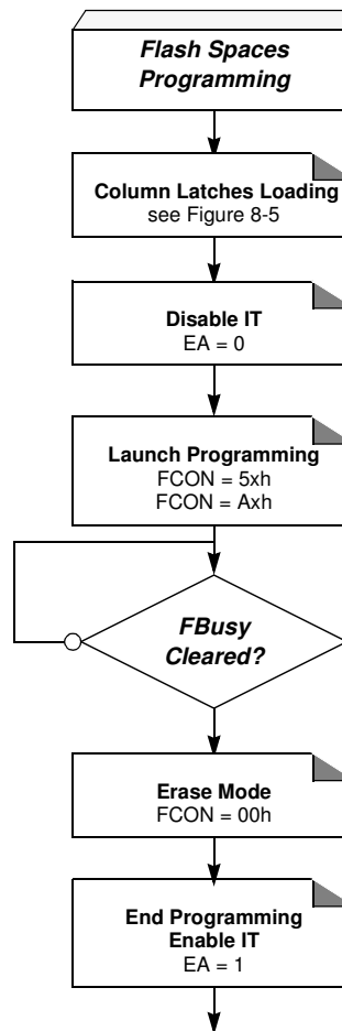
Figure 8-6. Flash and Extra Row Programming Procedure
