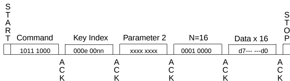
Figure 8-16. Verify Crypto
