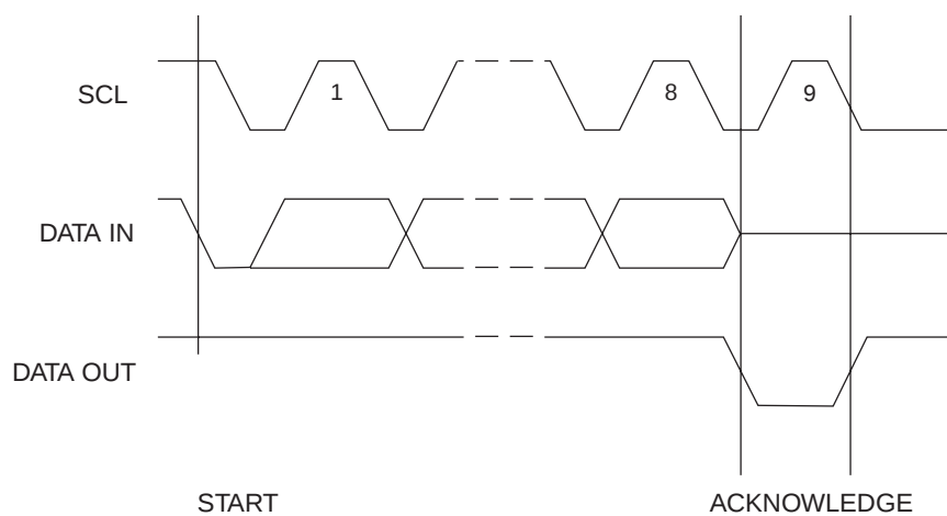
Figure 12-5. Output Acknowledge
