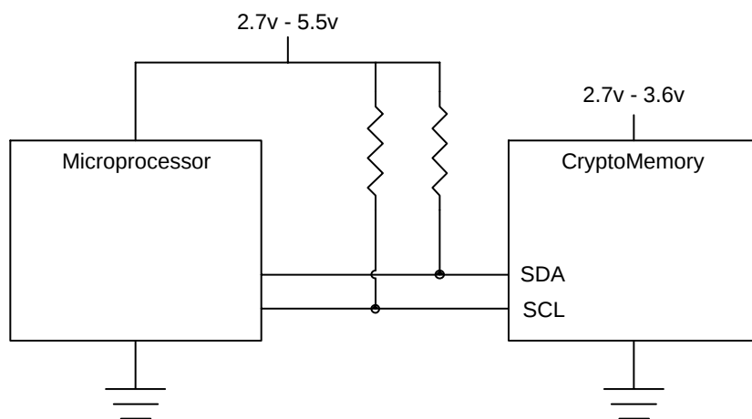
Figure 4-1. Connection Diagram
