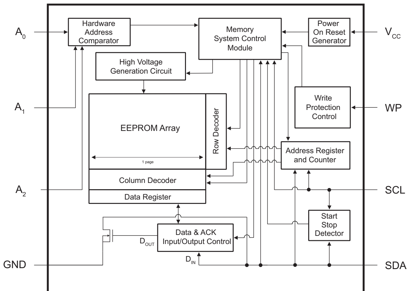
Figure 2-1. Block Diagram
