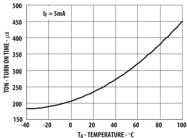
Figure 12: Typical Turn On Time vs. Temperature
