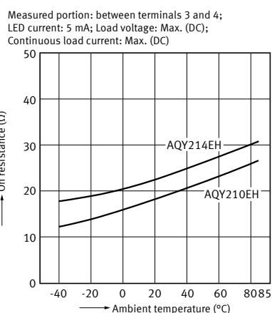
2-1. On resistance vs. ambient temperature characteristics
