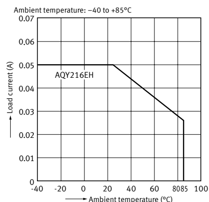
1-3. Load current vs. ambient temperature characteristics
