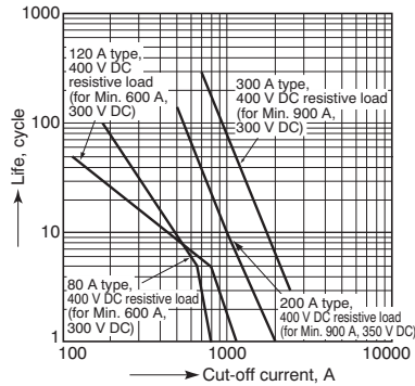
4. Cut-off life curve (Forward direction)
