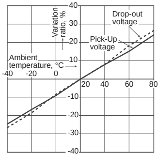
1.-(2) Ambient temperature characteristics (20 A type) Sample: EV relay 20 A, 3 pcs.
