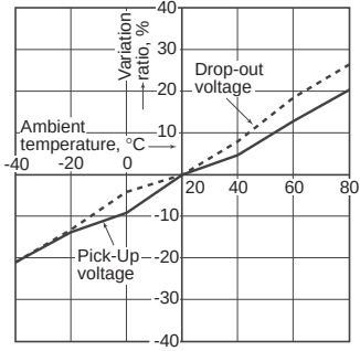
1.-(3) Ambient temperature characteristics (80 A type) Sample: EV relay 80 A, 3 pcs.
