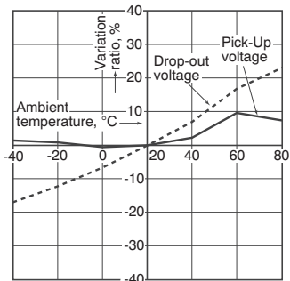
1.-(6) Ambient temperature characteristics (300 A type) Sample: EV relay 300 A, 3 pcs.
