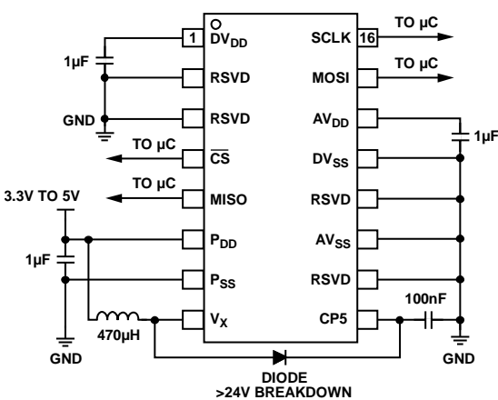
Figure 15. Recommended ADXRS810 Application Circuit
