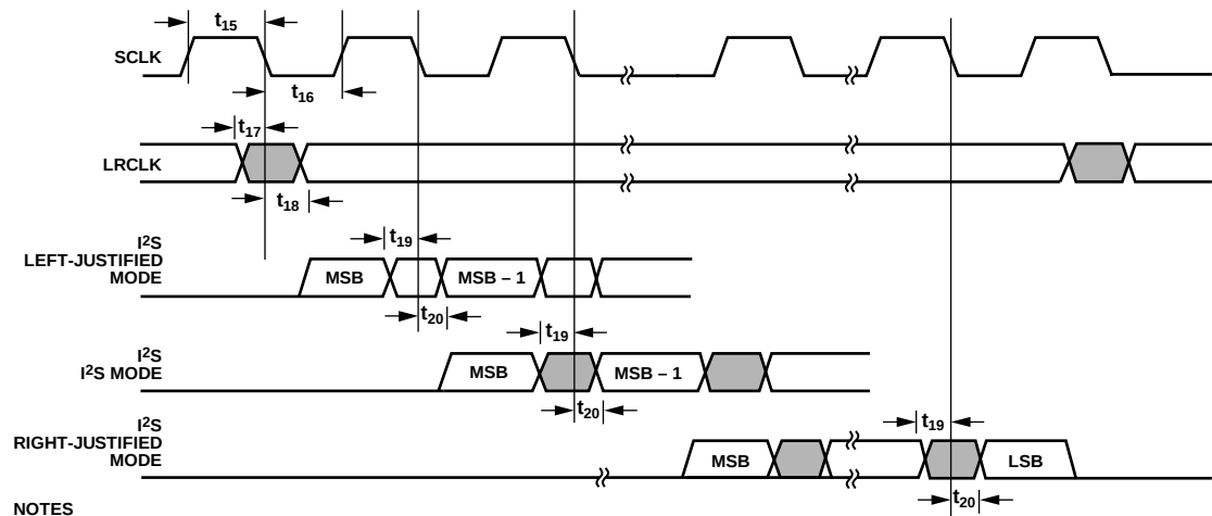
Figure 5. I²S Timing
