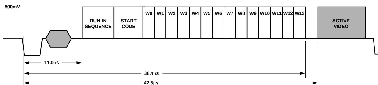
Figure 58. WSS Waveform Diagram
