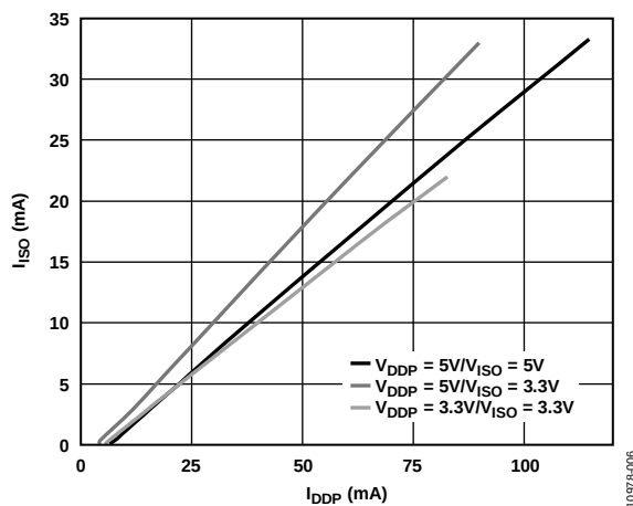
Figure 6. Typical Isolated Output Supply Current, I_{ISO} , as a Function of External Load, at 5 V/5 V, 5 V/3.3 V, and 3.3 V/3.3 V
