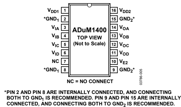
Figure 5. ADuM1400 Pin Configuration
