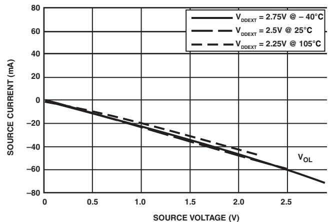
Figure 29. Driver Type B Current ( 2.5V_{DDEXT} )
