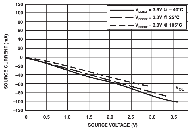
Figure 28. Driver Type B Current ( 3.3V_{DDEXT} )
