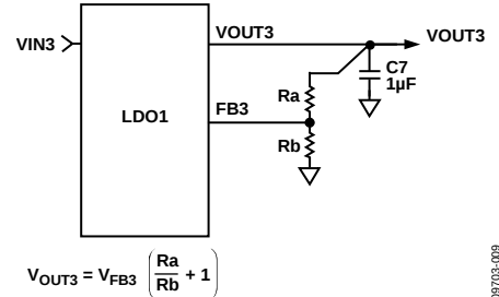
Figure 49. LDO1 External Output Voltage Setting
