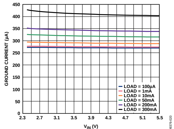
Figure 40. Ground Current vs. Input Voltage, V_{\text{OUTx}} = 1.2\text{ V} and 1.8\text{ V} , Dual Output, Includes 200 \mu\text{A} for Output Dividers, ADP223/ADP225
