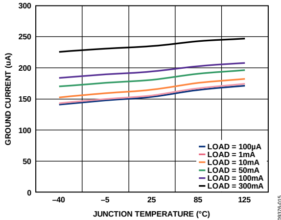
Figure 35. Ground Current vs. Junction Temperature, Single Output, Includes 100 \mu\text{A} for Output Divider, ADP223/ADP225
