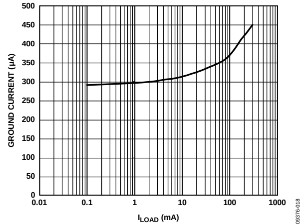
Figure 38. Ground Current vs. Load Current, Dual Output, Includes 200 \mu\text{A} for Output Dividers, ADP223/ADP225
