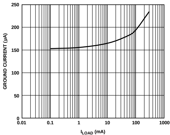
Figure 37. Ground Current vs. Load Current, Single Output, Includes 100 \mu\text{A} for Output Divider, ADP223/ADP225
