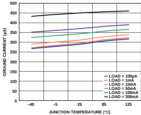
Figure 36. Ground Current vs. Junction Temperature, Dual Output, Includes 200 \mu\text{A} for Output Dividers, ADP223/ADP225
