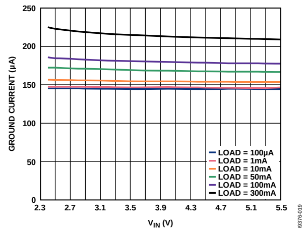
Figure 39. Ground Current vs. Input Voltage, V_{\text{OUTx}} = 1.2\text{ V} , Single Output, Includes 100 \mu\text{A} for Output Divider, ADP223/ADP225
