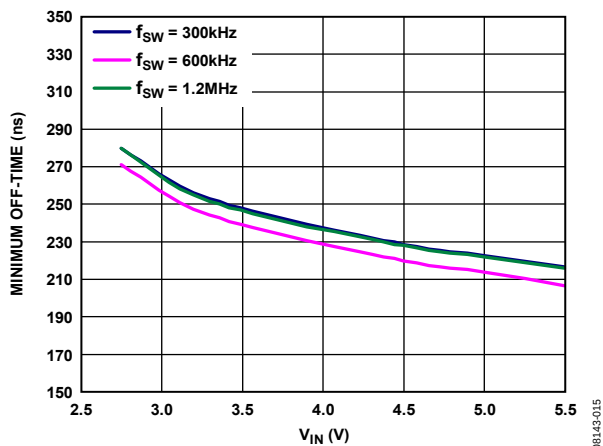
Figure 15. Minimum Off-Time, Open Loop, Includes Dead Time
