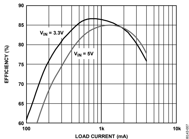
Figure 7. Efficiency Combined Dual-Phase Output, V_{OUT} = 0.8V and f_{SW} = 1.2\text{ MHz} ; Inductor TOKO FDV0620-1R0M, 1.0\text{ }\mu\text{H} , 14\text{ m}\Omega
