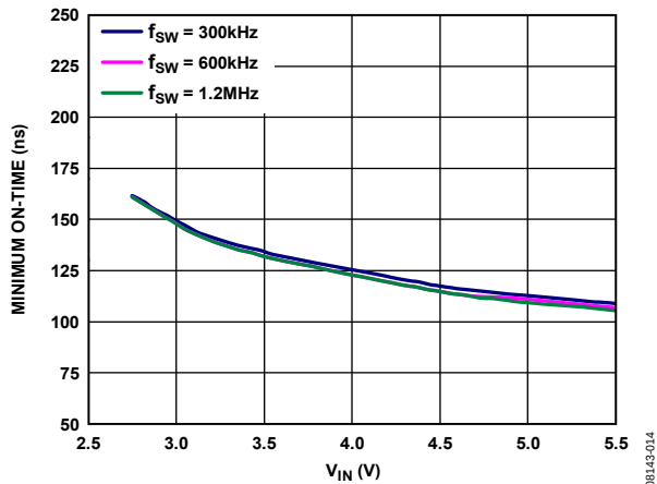
Figure 14. Minimum On-Time, Open Loop, Includes Dead Time
