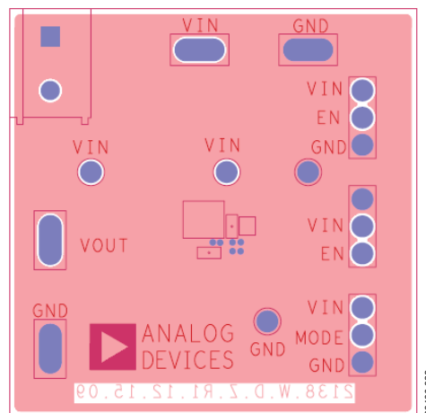
Figure 38. Bottom Layer
