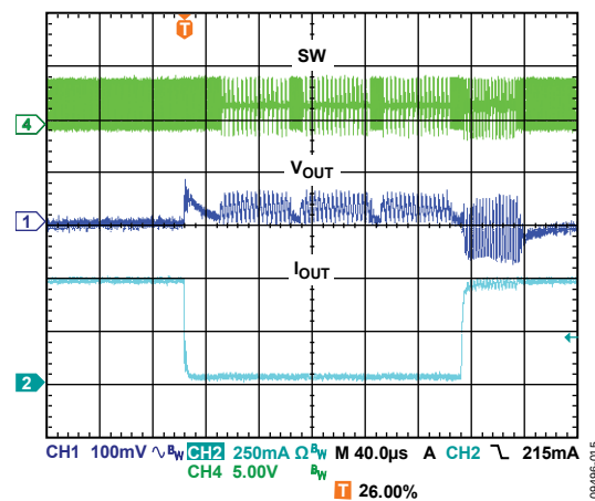
Figure 18. Response to Load Transient, 50 mA to 500 mA, V_{OUT} = 1.8 V, Automatic Mode
