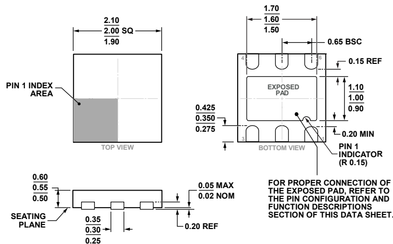
Figure 35. 6-Lead Lead Frame Chip Scale Package [LFCSP_UD] 2.00 mm × 2.00 mm Body, Ultra Thin, Dual Lead
