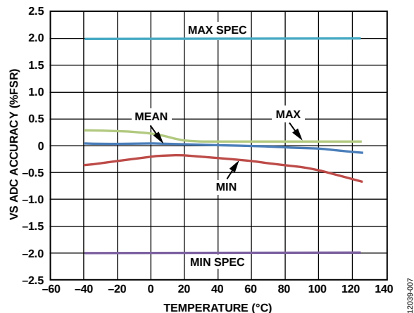
Figure 4. VS ADC Accuracy vs. Temperature (From 10% to 90% of FSR)
