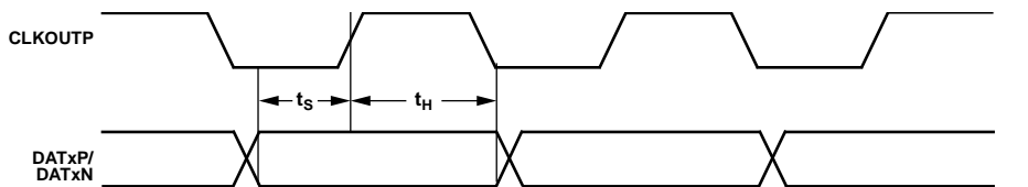
Figure 6. Nibble Output Mode (Full Rate Clock)
