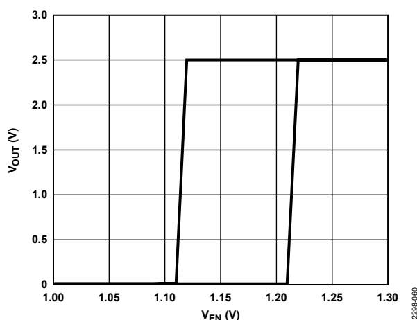
Figure 58. Typical V OUT Response to EN Pin Operation
