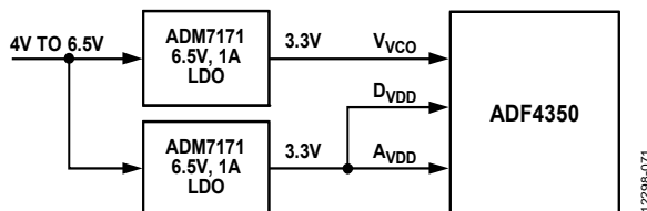
Figure 68. RF PLL/VCO Power
