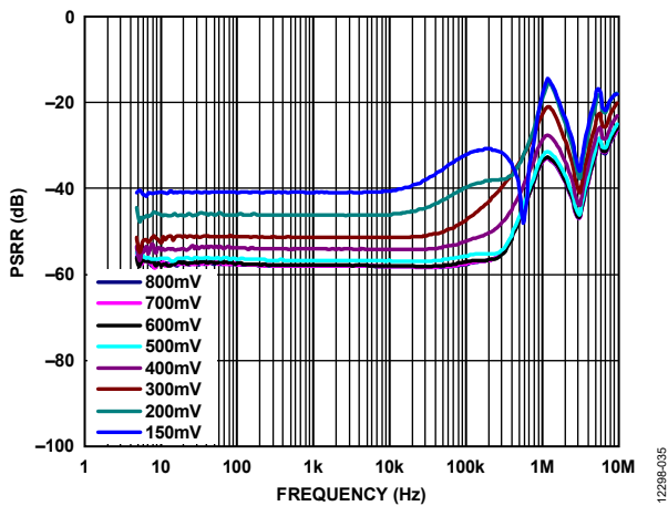
Figure 35. Power Supply Rejection Ratio (PSRR) vs. Frequency, V_{OUT} = 5\text{ V} , 1 A Load Current, Various Headroom Voltages
