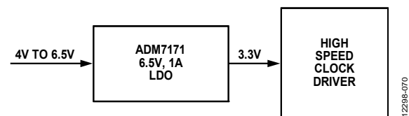
Figure 67. Clock Driver Power
