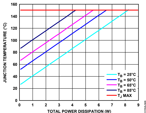
Figure 66. LFCSP Power Dissipation for Various Board Temperatures
